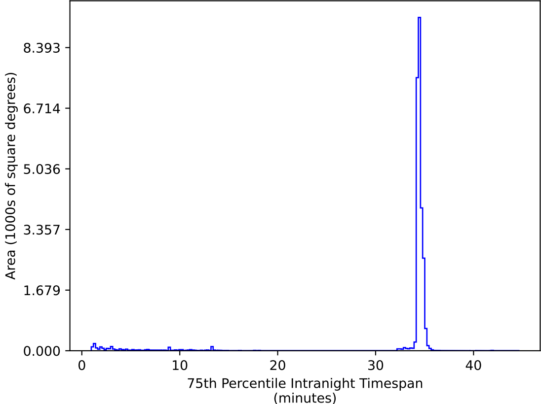
too_elab_r64_d3_ugrizy_v3.4_10yrs All sky zy bands: 75th Percentile Intranight Timespan
