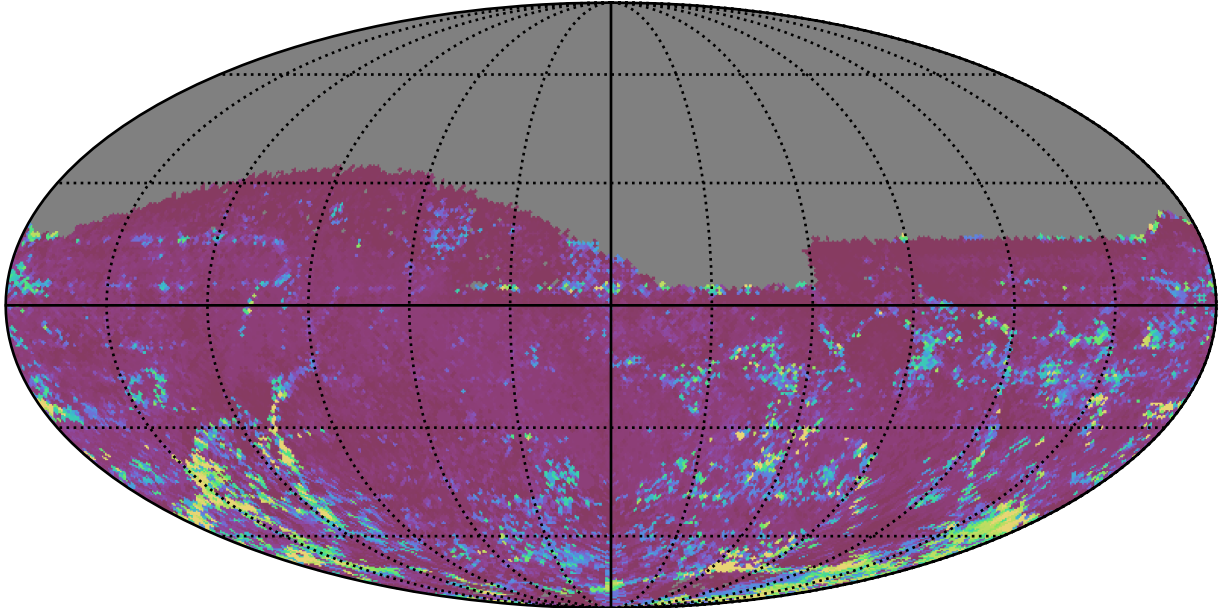
too_elab_r64_d3_ugrizy_v3.4_10yrs All sky z band: 75th Percentile Intranight Timespan
