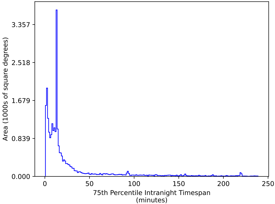
too_elab_r64_d3_ugrizy_v3.4_10yrs All sky z band: 75th Percentile Intranight Timespan
