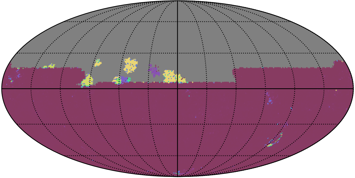
too_elab_r64_d3_ugrizy_v3.4_10yrs All sky y band: 75th Percentile Intranight Timespan
