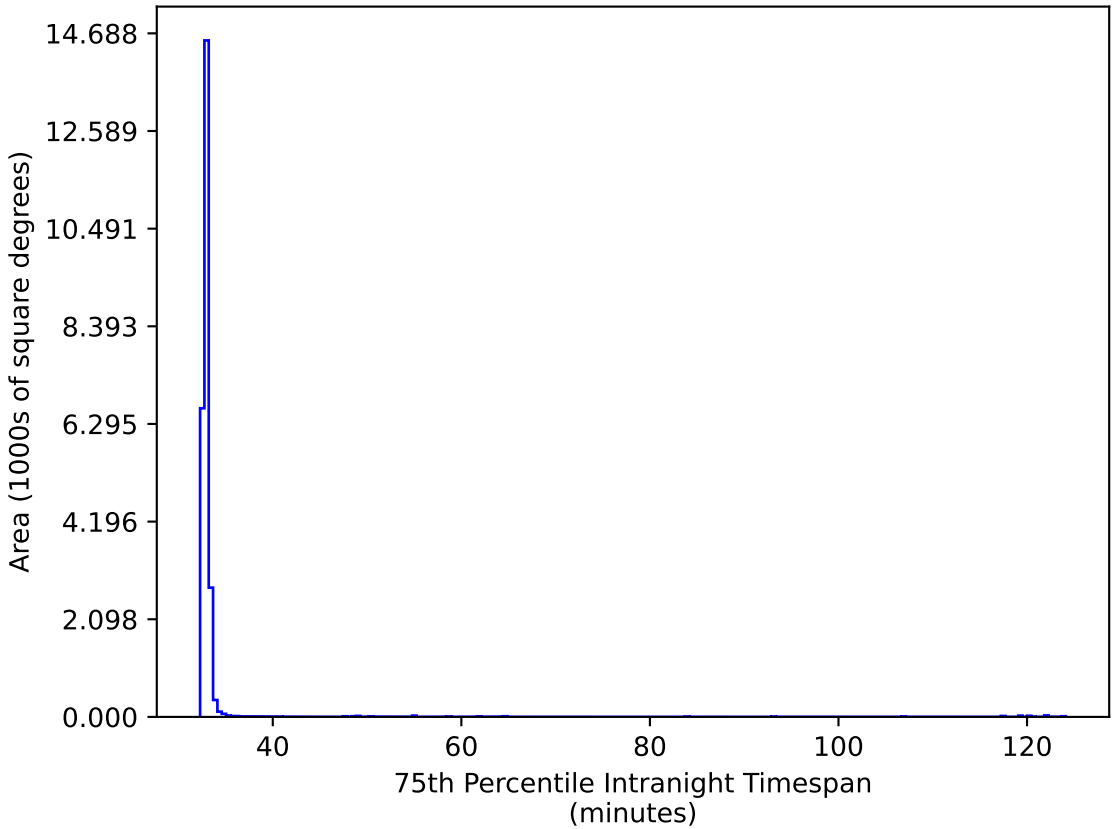
too_elab_r64_d3_ugrizy_v3.4_10yrs All sky y band: 75th Percentile Intranight Timespan
