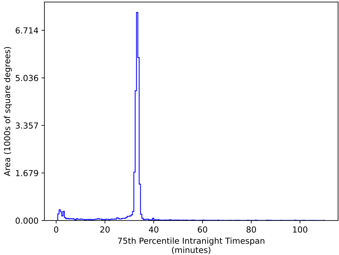
too_elab_r64_d3_ugrizy_v3.4_10yrs All sky ug bands: 75th Percentile Intranight Timespan
