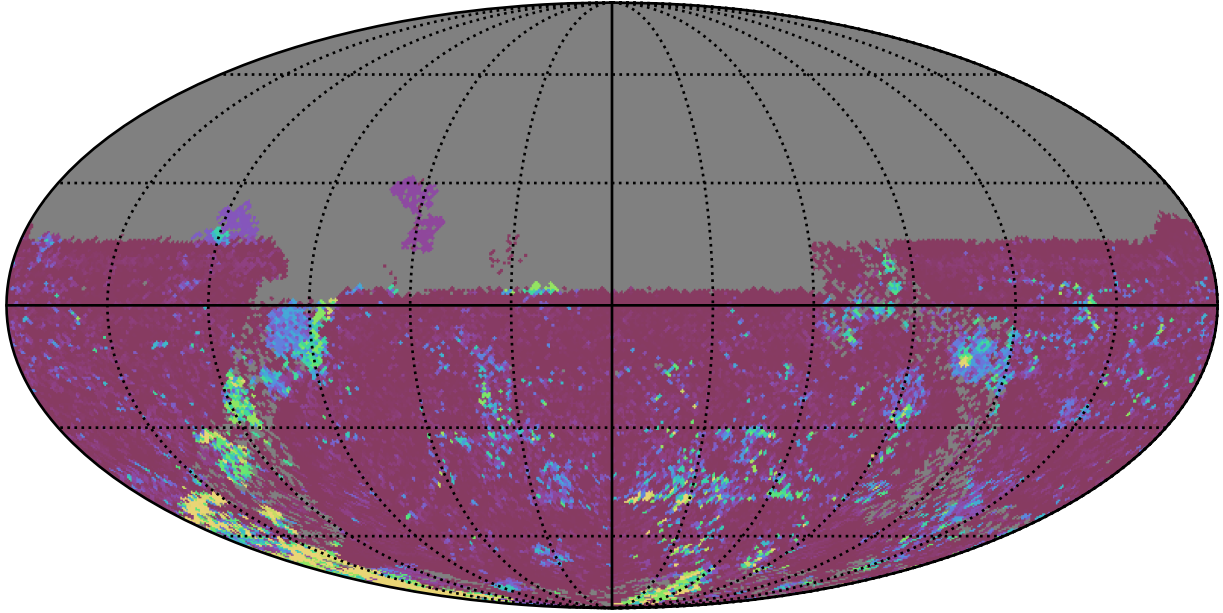
too_elab_r64_d3_ugrizy_v3.4_10yrs All sky u band: 75th Percentile Intranight Timespan
