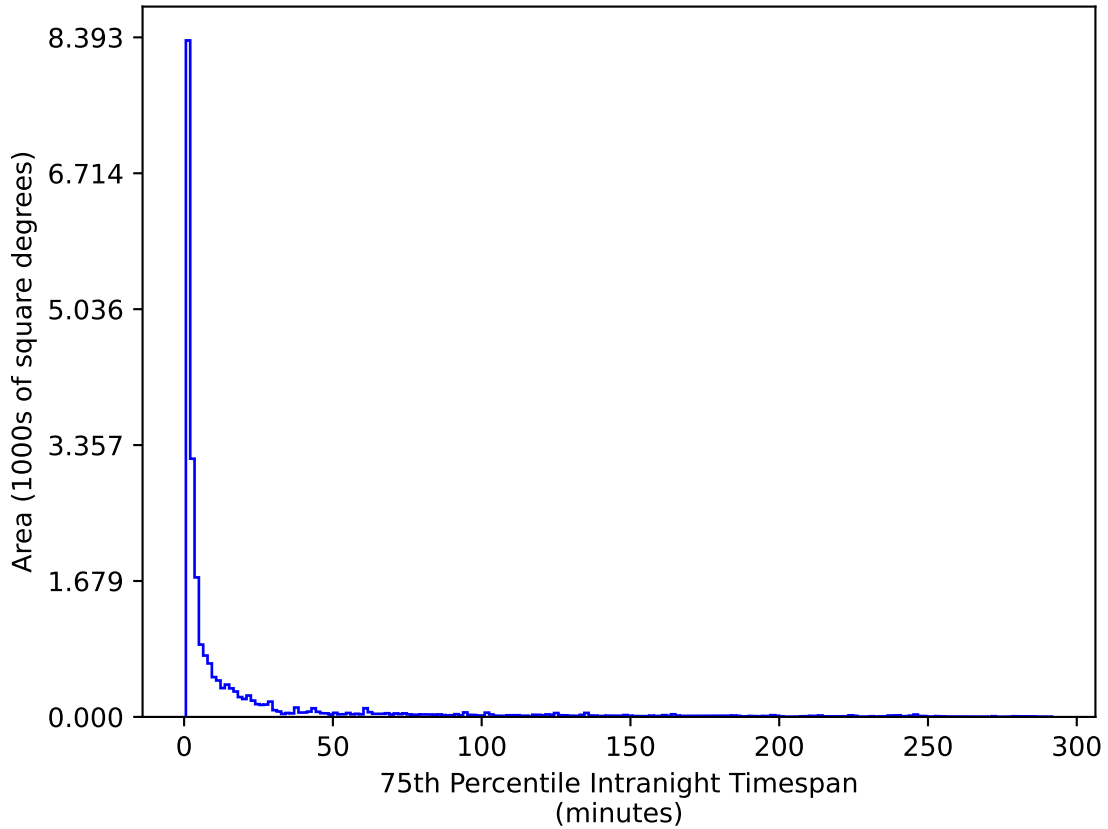
too_elab_r64_d3_ugrizy_v3.4_10yrs All sky u band: 75th Percentile Intranight Timespan
