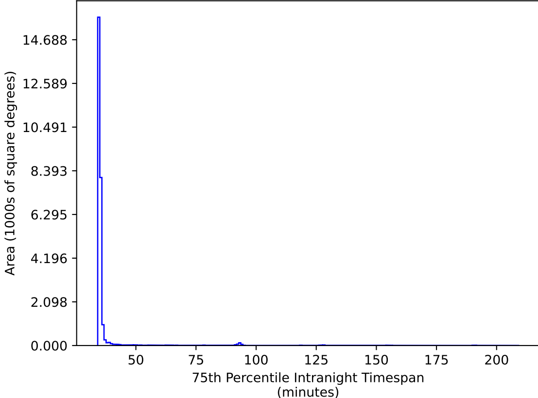
too_elab_r64_d3_ugrizy_v3.4_10yrs All sky ri bands: 75th Percentile Intranight Timespan
