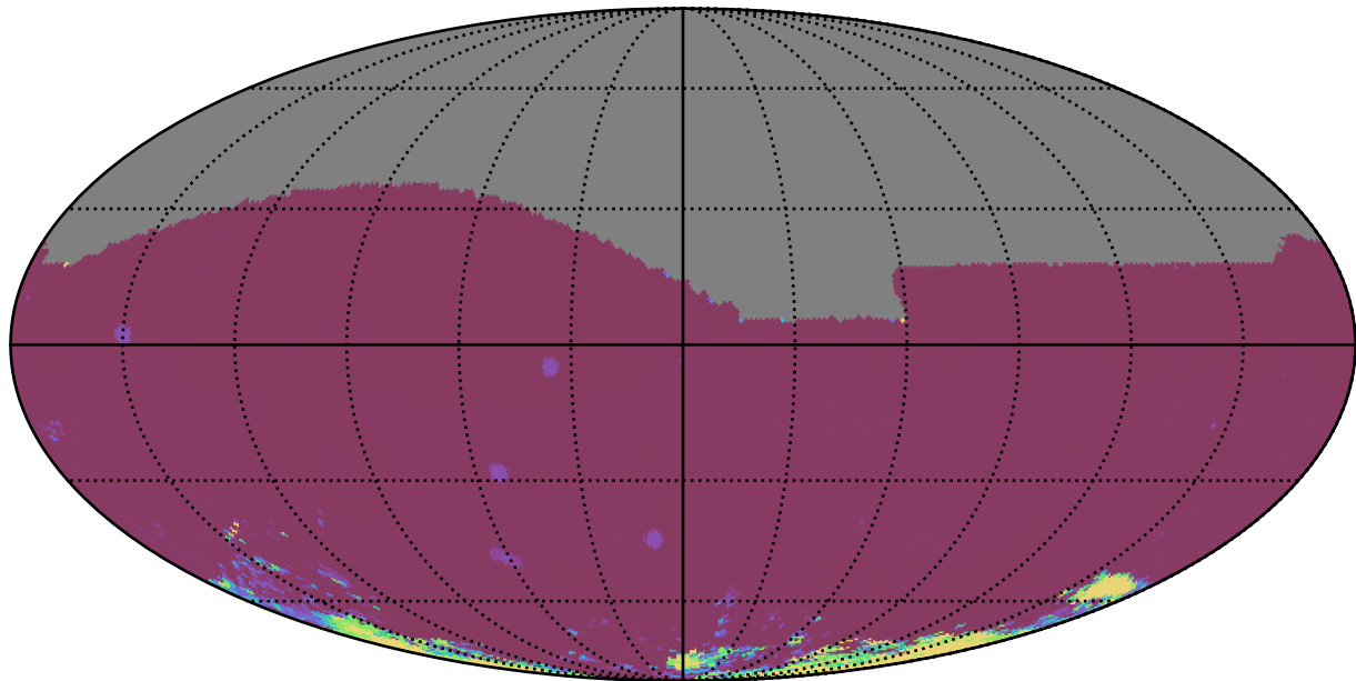
too_elab_r64_d3_ugrizy_v3.4_10yrs All sky iz bands: 75th Percentile Intranight Timespan
