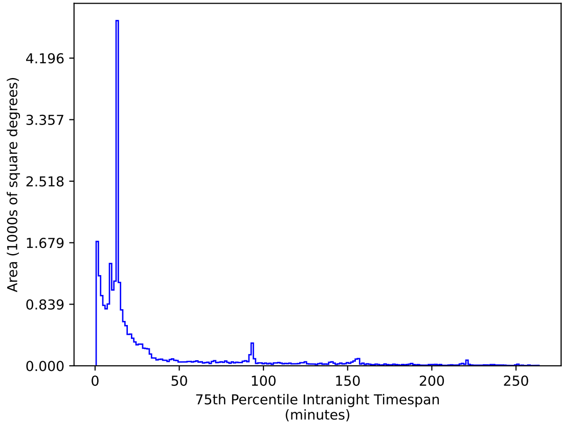
too_elab_r64_d3_ugrizy_v3.4_10yrs All sky i band: 75th Percentile Intranight Timespan
