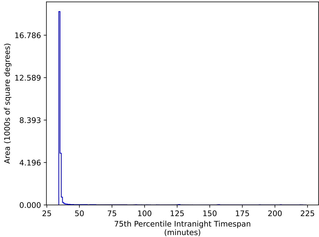
too_elab_r64_d3_ugrizy_v3.4_10yrs All sky gr bands: 75th Percentile Intranight Timespan
