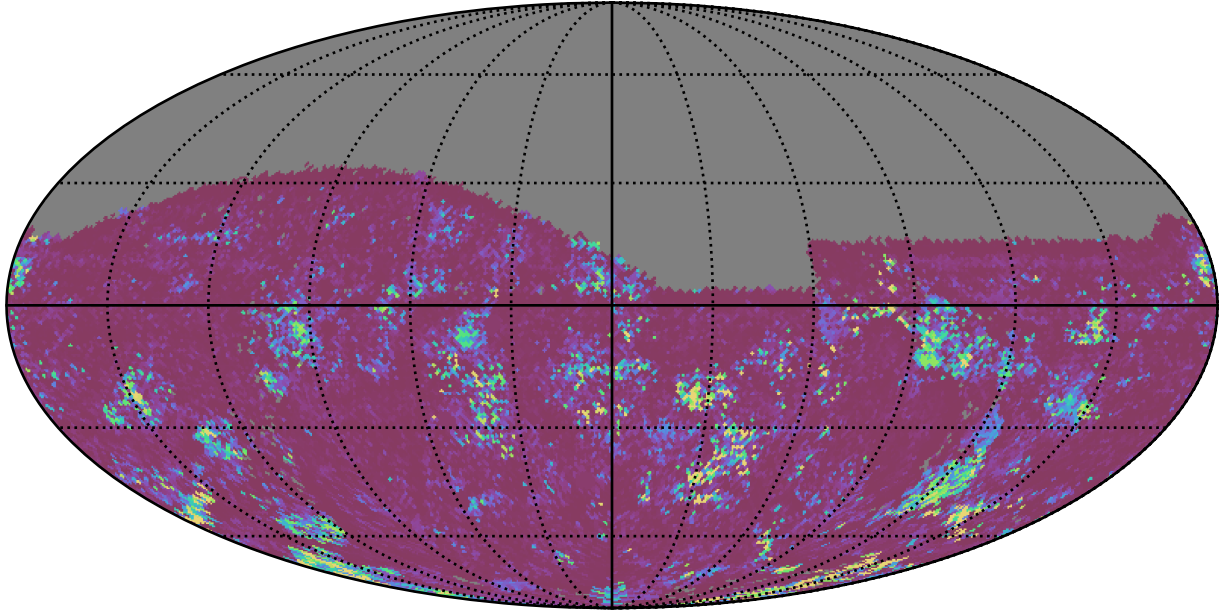
too_elab_r64_d3_ugrizy_v3.4_10yrs All sky g band: 75th Percentile Intranight Timespan
