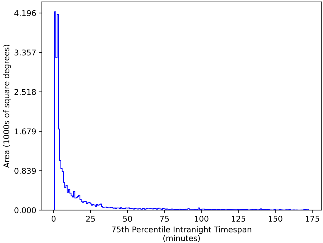
too_elab_r64_d3_ugrizy_v3.4_10yrs All sky g band: 75th Percentile Intranight Timespan
