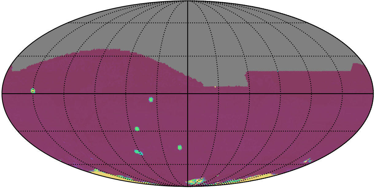
too_elab_r64_d3_ugrizy_v3.4_10yrs All sky all bands: 75th Percentile Intranight Timespan
