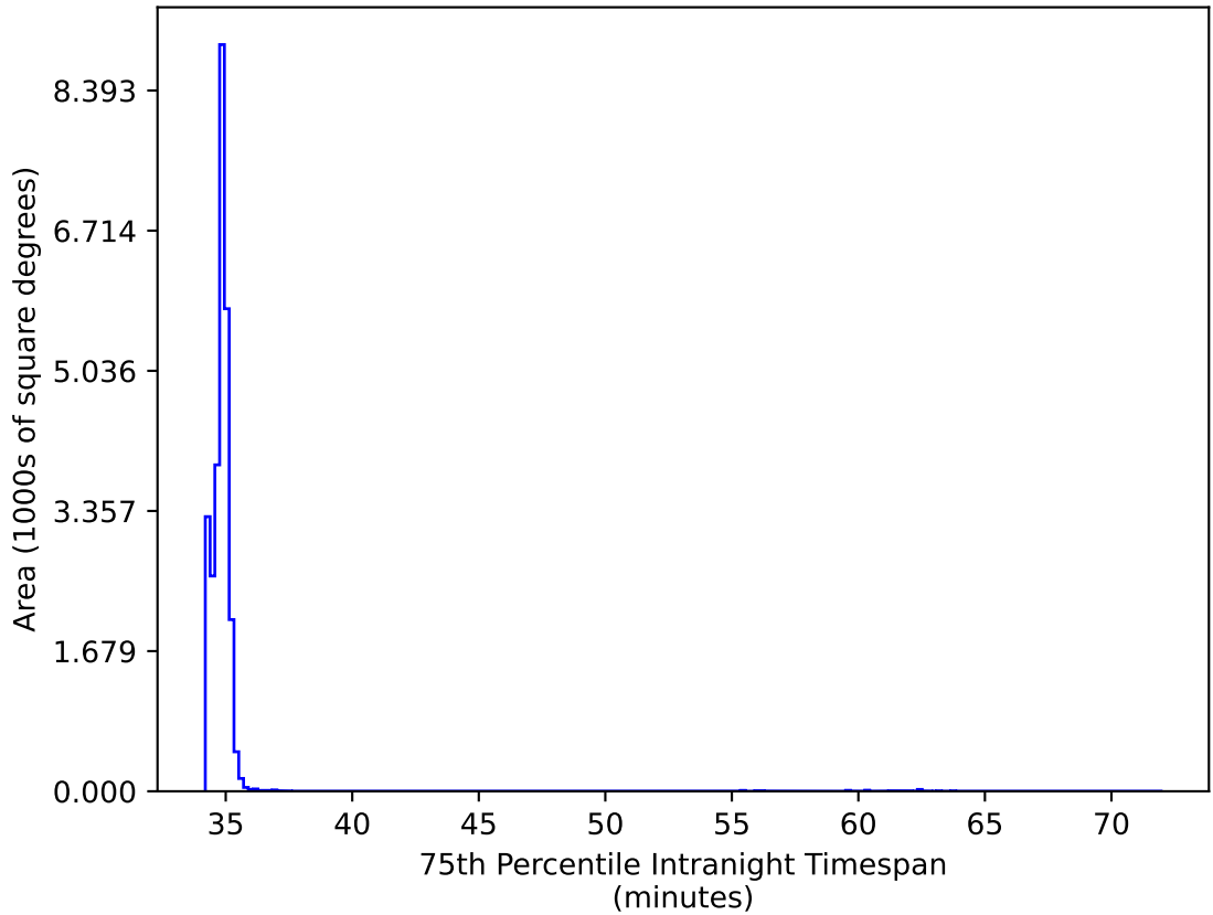
too_elab_r64_d3_ugrizy_v3.4_10yrs All sky: 75th Percentile Intranight Timespan
