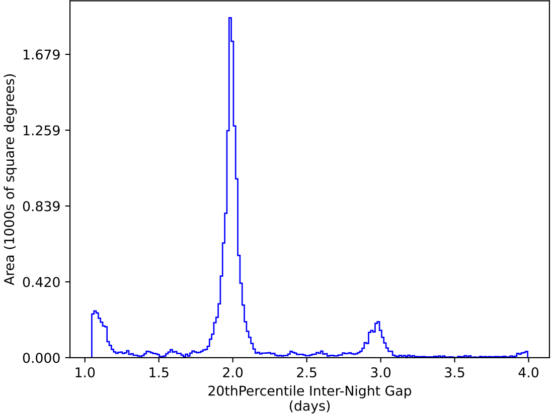
too_elab_r64_d3_ugrizy_v3.4_10yrs WFD y band: 20thPercentile Inter-Night Gap
