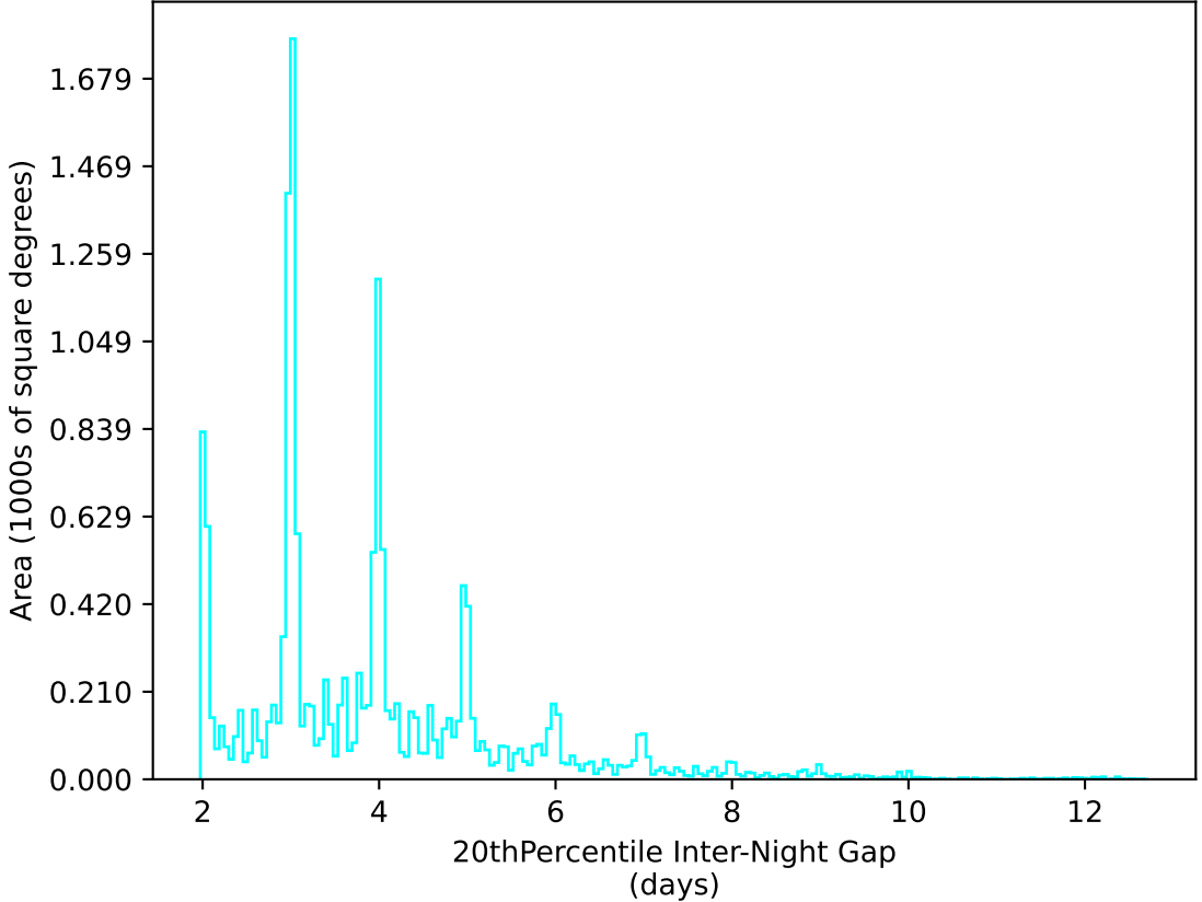
too_elab_r64_d3_ugrizy_v3.4_10yrs WFD u band: 20thPercentile Inter-Night Gap
