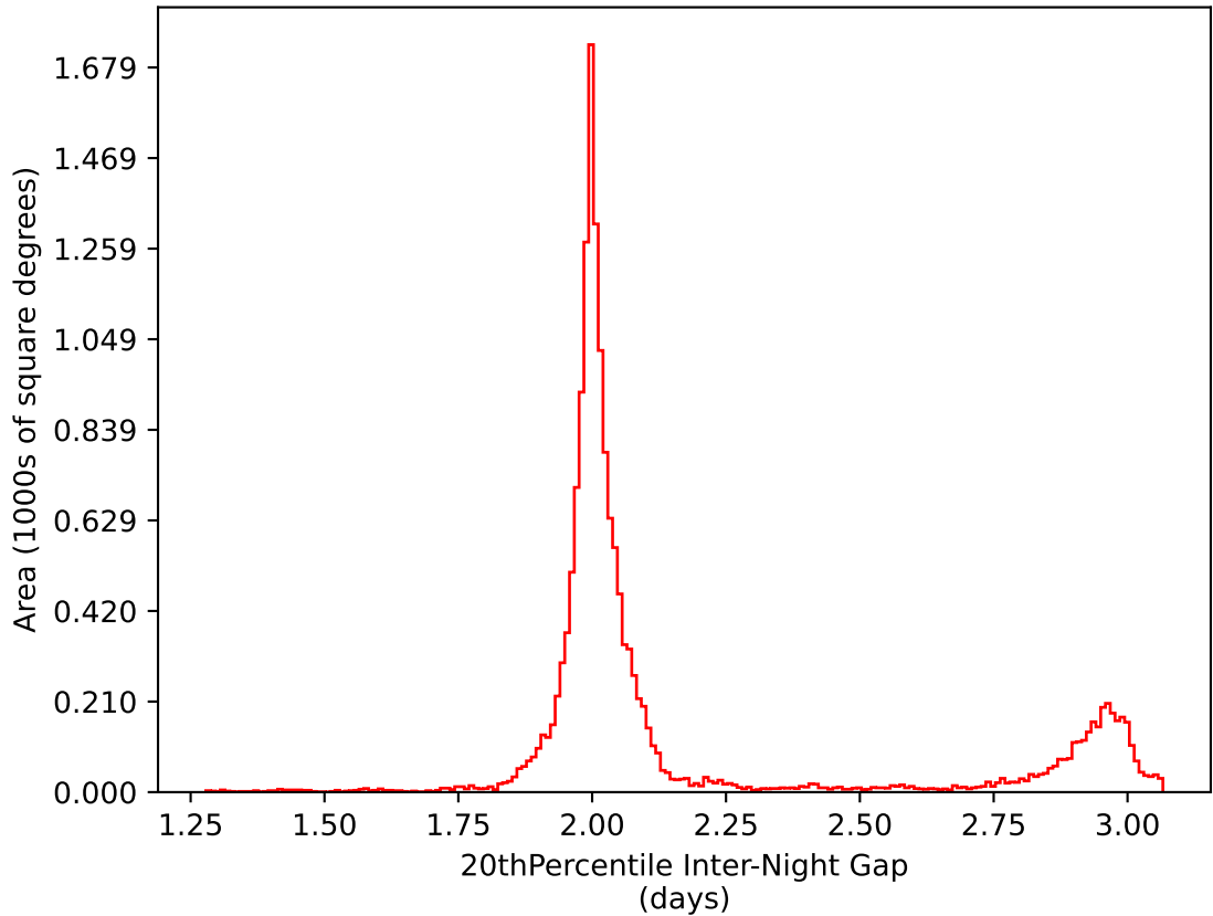
too_elab_r64_d3_ugrizy_v3.4_10yrs WFD i band: 20thPercentile Inter-Night Gap
