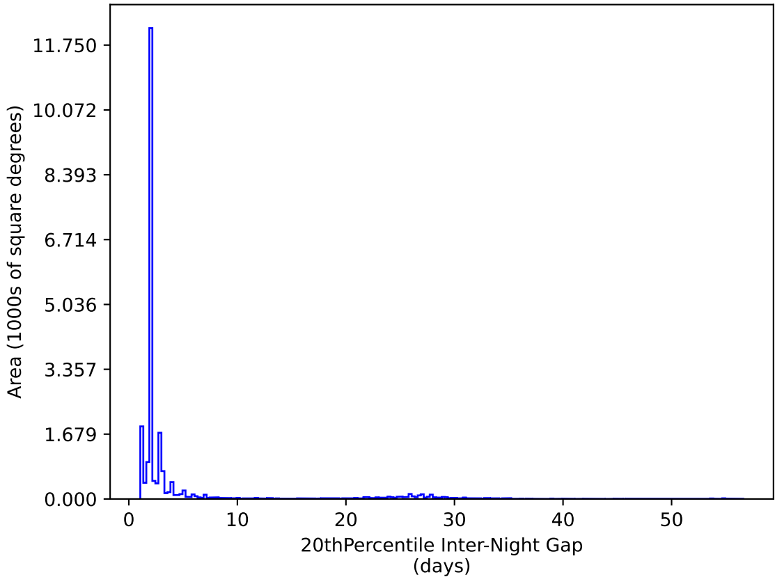
too_elab_r64_d3_ugrizy_v3.4_10yrs All sky y band: 20thPercentile Inter-Night Gap
