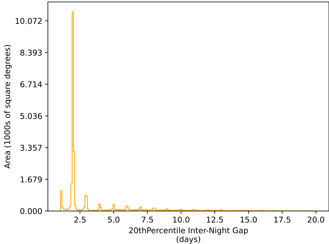
too_elab_r64_d3_ugrizy_v3.4_10yrs All sky r band: 20thPercentile Inter-Night Gap
