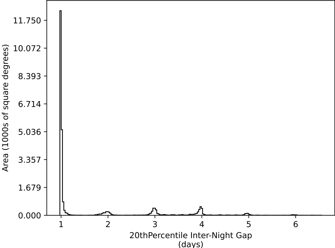
too_elab_r64_d3_ugrizy_v3.4_10yrs All sky all bands: 20thPercentile Inter-Night Gap
