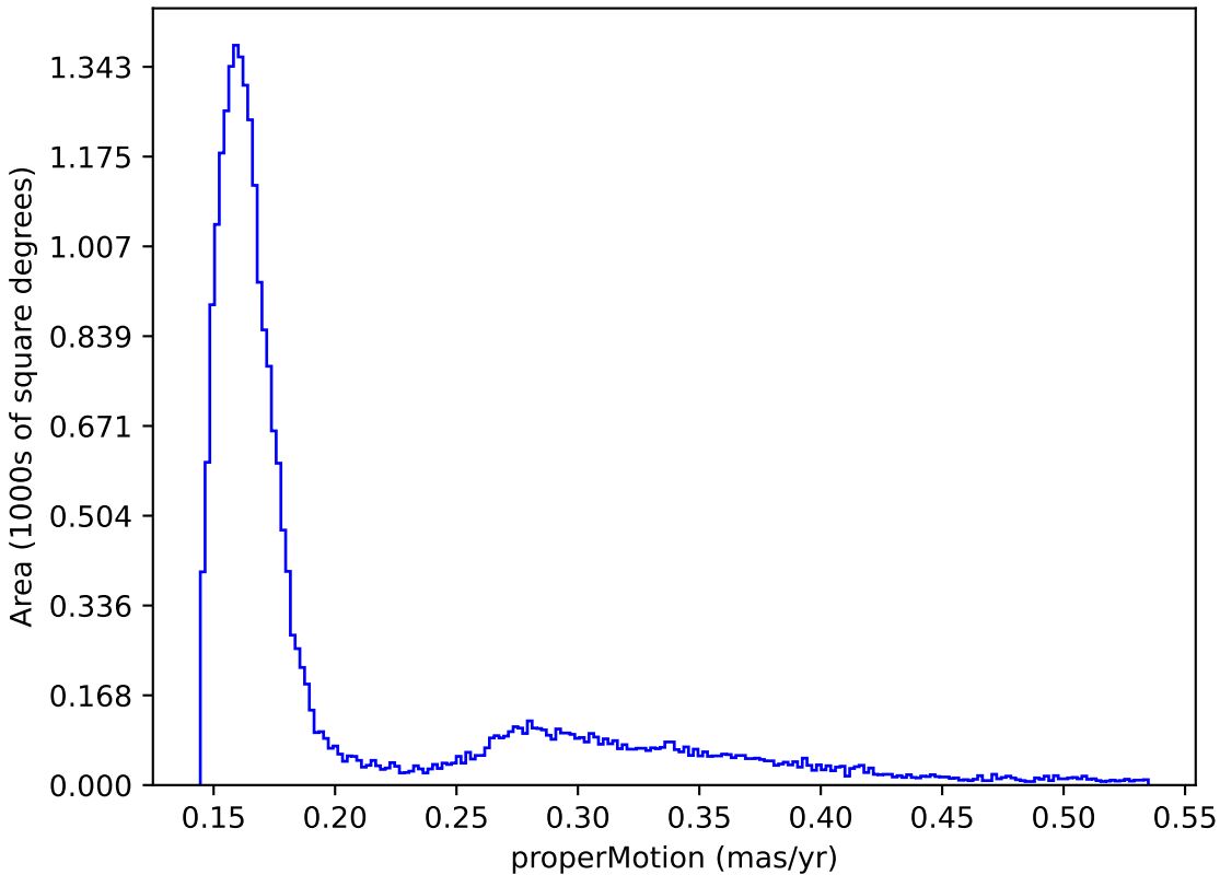
too_elab_r64_d3_ugrizy_v3.4_10yrs : properMotion
