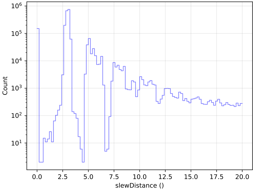
too_elab_r64_d3_ugrizy_v3.4_10yrs All visits: Zoom Slew Distance Histogram
