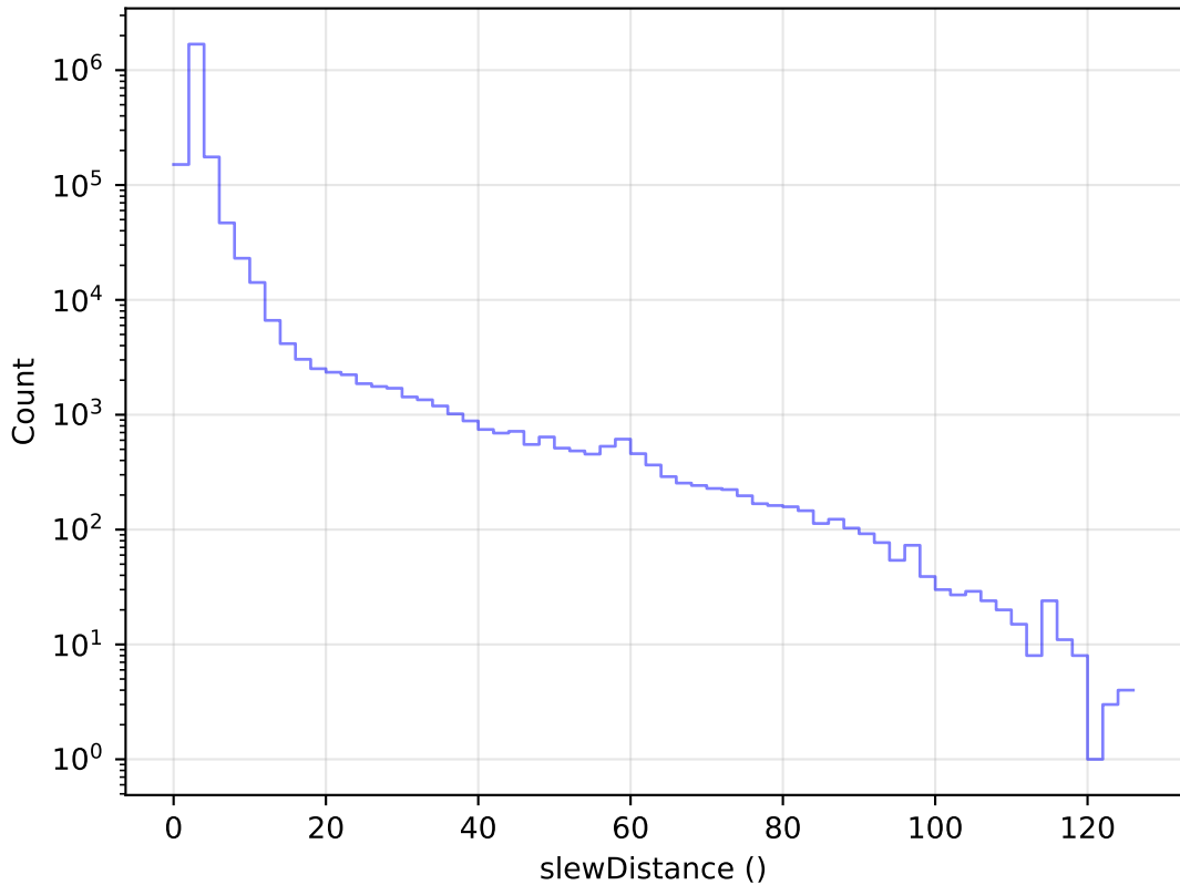
too_elab_r64_d3_ugrizy_v3.4_10yrs All visits: Slew Distance Histogram
