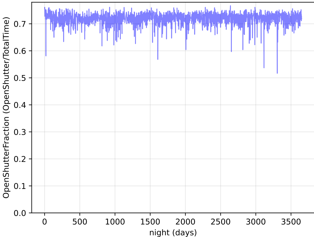
too_elab_r64_d3_ugrizy_v3.4_10yrs : OpenShutterFraction
