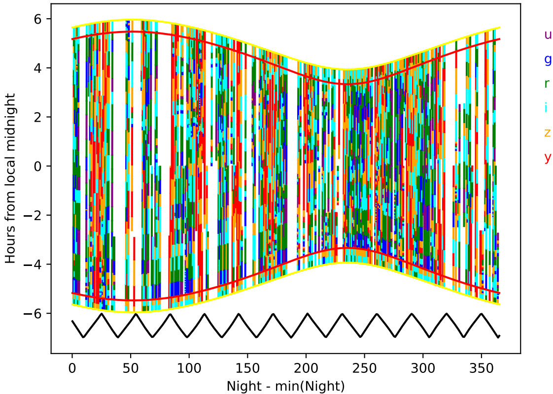
too_elab_r64_d3_ugrizy_v3.4_10yrs year 7-8: Hourglass
