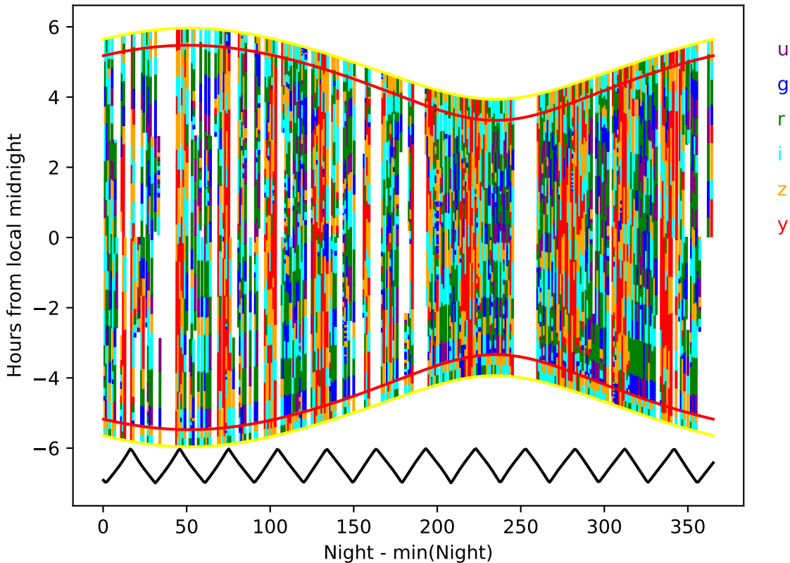
too_elab_r64_d3_ugrizy_v3.4_10yrs year 5-6: Hourglass
