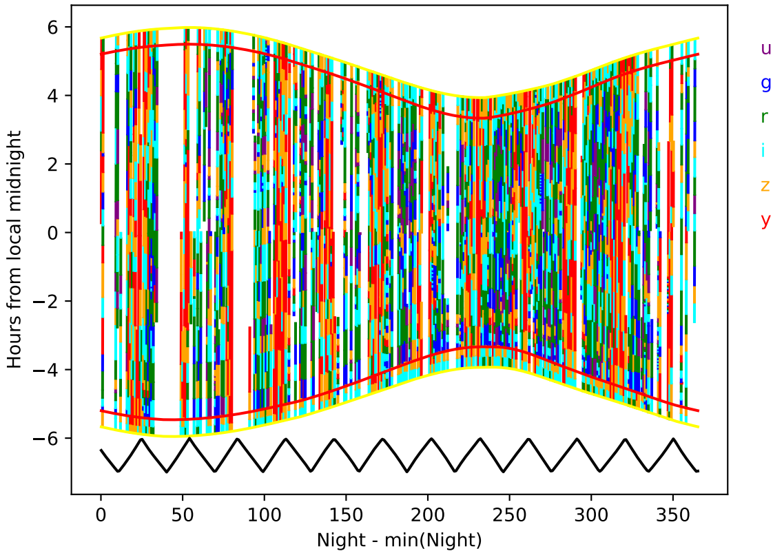
too_elab_r64_d3_ugrizy_v3.4_10yrs year 4-5: Hourglass
