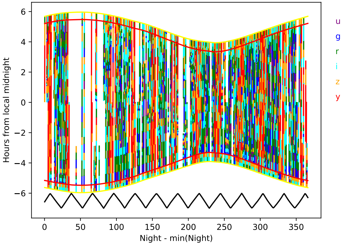
too_elab_r64_d3_ugrizy_v3.4_10yrs_year 3-4: Hourglass
