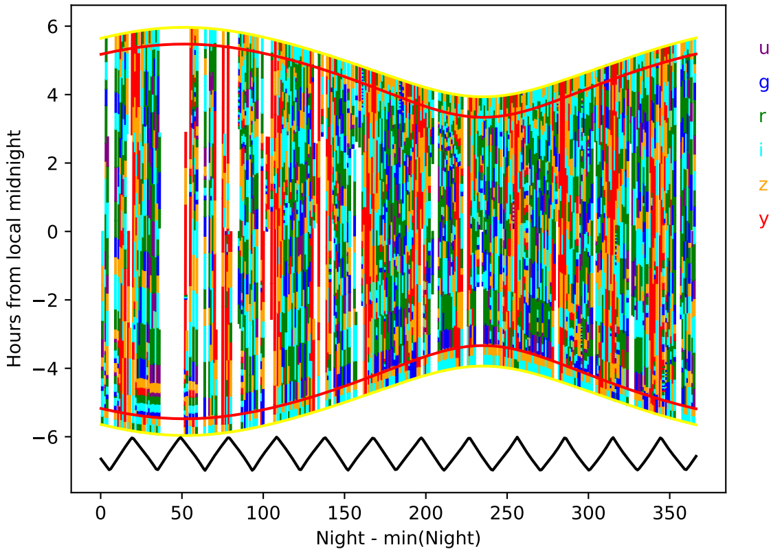
too_elab_r64_d3_ugrizy_v3.4_10yrs_year 2-3: Hourglass
