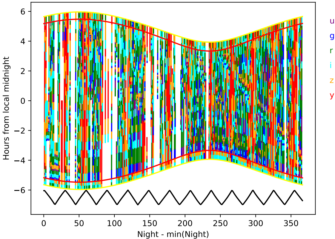
too_elab_r64_d3_ugrizy_v3.4_10yrs year 1-2: Hourglass
