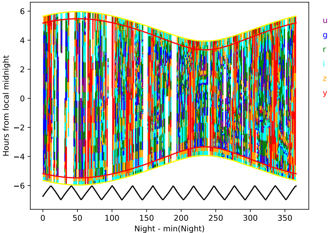
too_elab_r64_d3_ugrizy_v3.4_10yrs year 0-1: Hourglass
