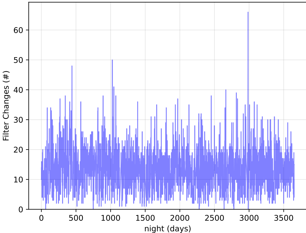
too_elab_r64_d3_ugrizy_v3.4_10yrs : Filter Changes
