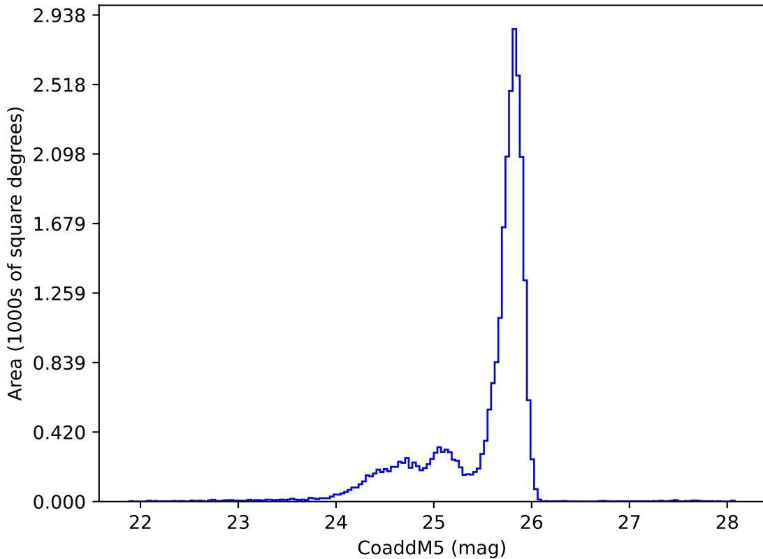
too_elab_r64_d3_ugrizy_v3.4_10yrs z: CoaddM5
