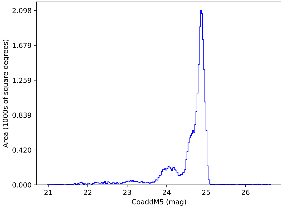
too_elab_r64_d3_ugrizy_v3.4_10yrs y: CoaddM5
