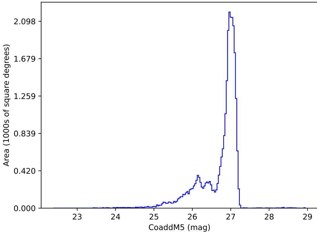
too_elab_r64_d3_ugrizy_v3.4_10yrs r: CoaddM5
