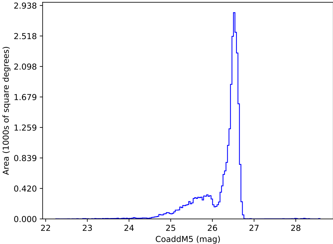
too_elab_r64_d3_ugrizy_v3.4_10yrs i: CoaddM5
