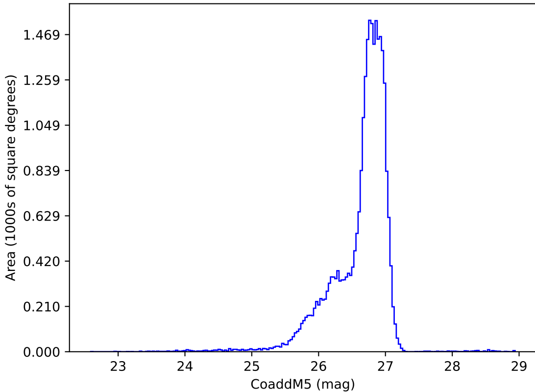
too_elab_r64_d3_ugrizy_v3.4_10yrs g: CoaddM5
