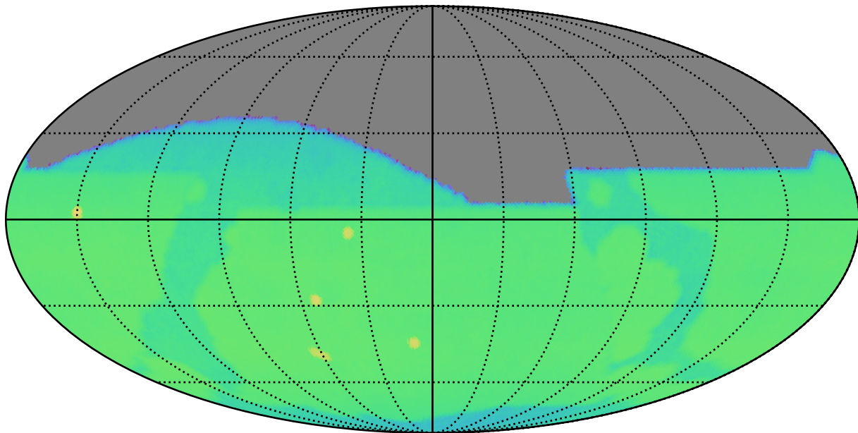
too_elab_r64_d3_ugrizy_v3.4_10yrs : CoaddM5
