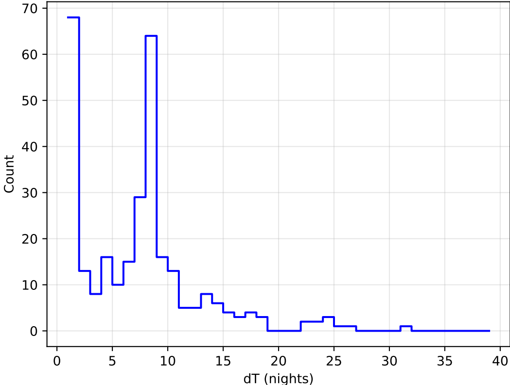
too_elab_r64_d3_ugrizy_v3.4_10yrs all bands: DD:XMM_LSS Delta Nights Histogram
