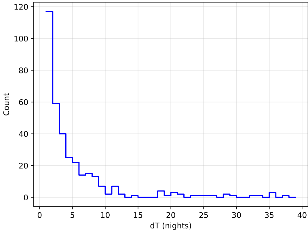
too_elab_r64_d3_ugrizy_v3.4_10yrs all bands: DD:WFD Delta Nights Histogram
