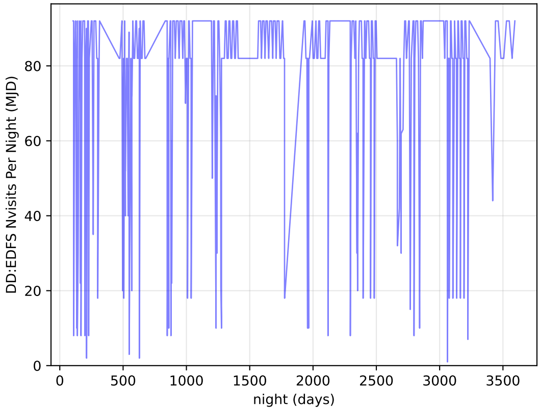
too_elab_r64_d3_ugrizy_v3.4_10yrs all bands: DD:EDFS Nvisits Per Night
