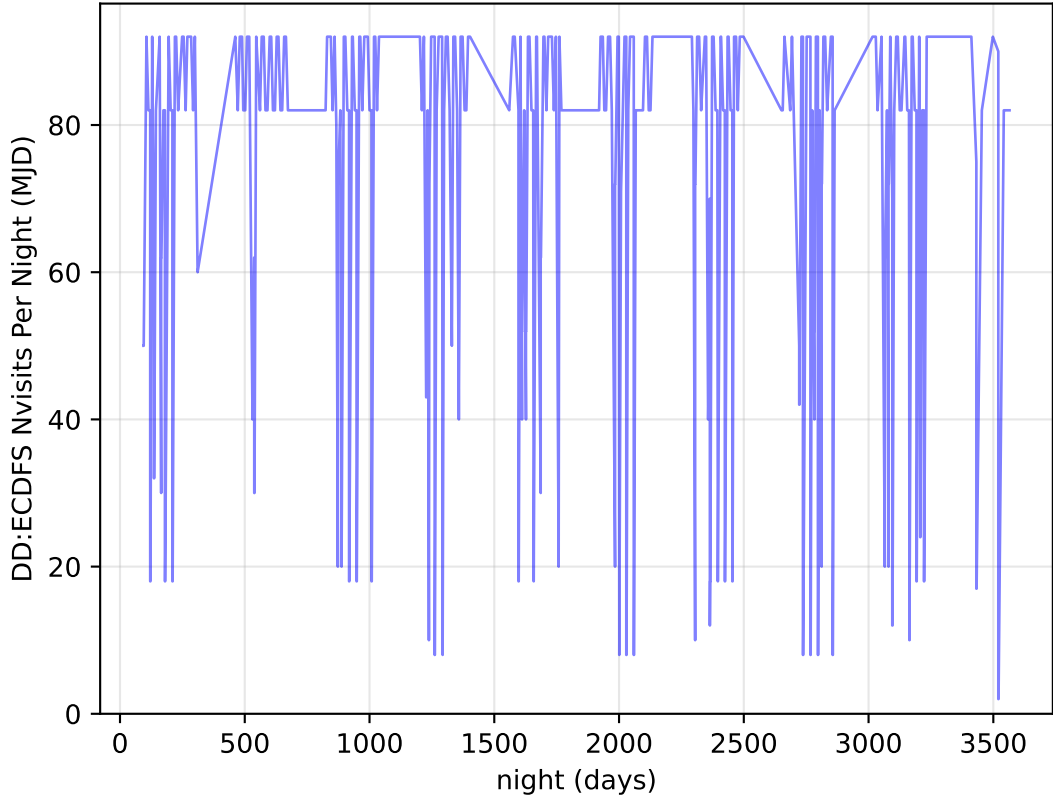
too_elab_r64_d3_ugrizy_v3.4_10yrs all bands: DD:ECDFS Nvisits Per Night
