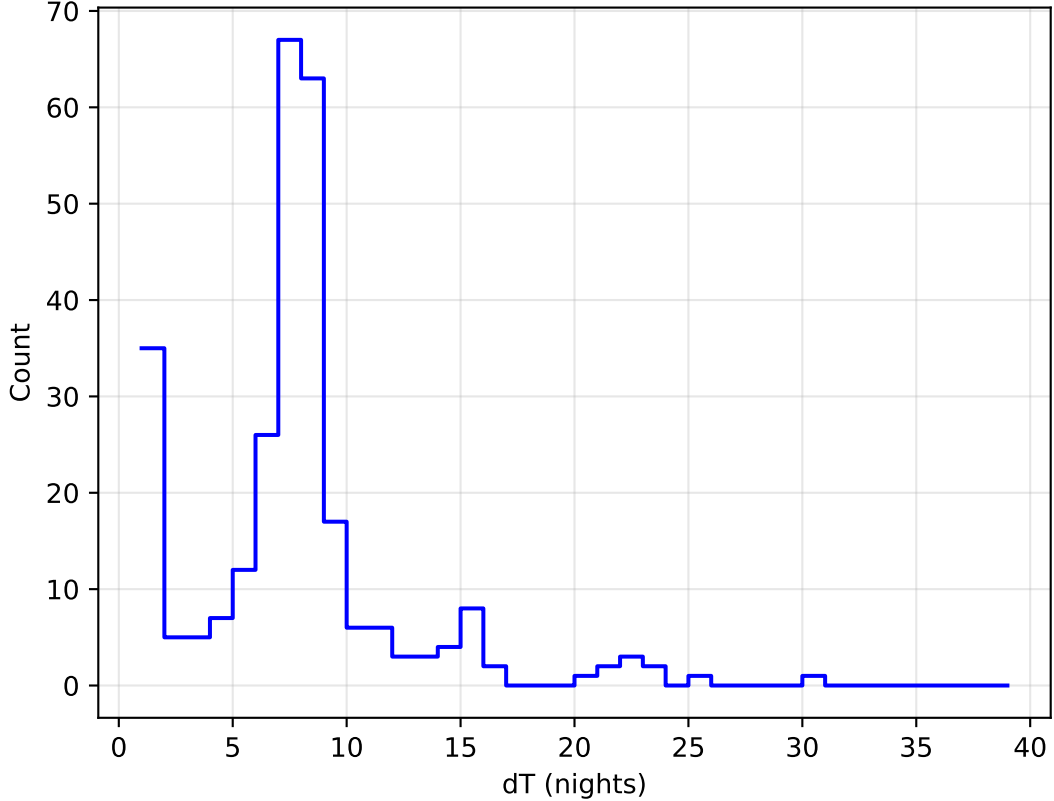
too_elab_r64_d3_ugrizy_v3.4_10yrs all bands: DD:ECDFS Delta Nights Histogram
