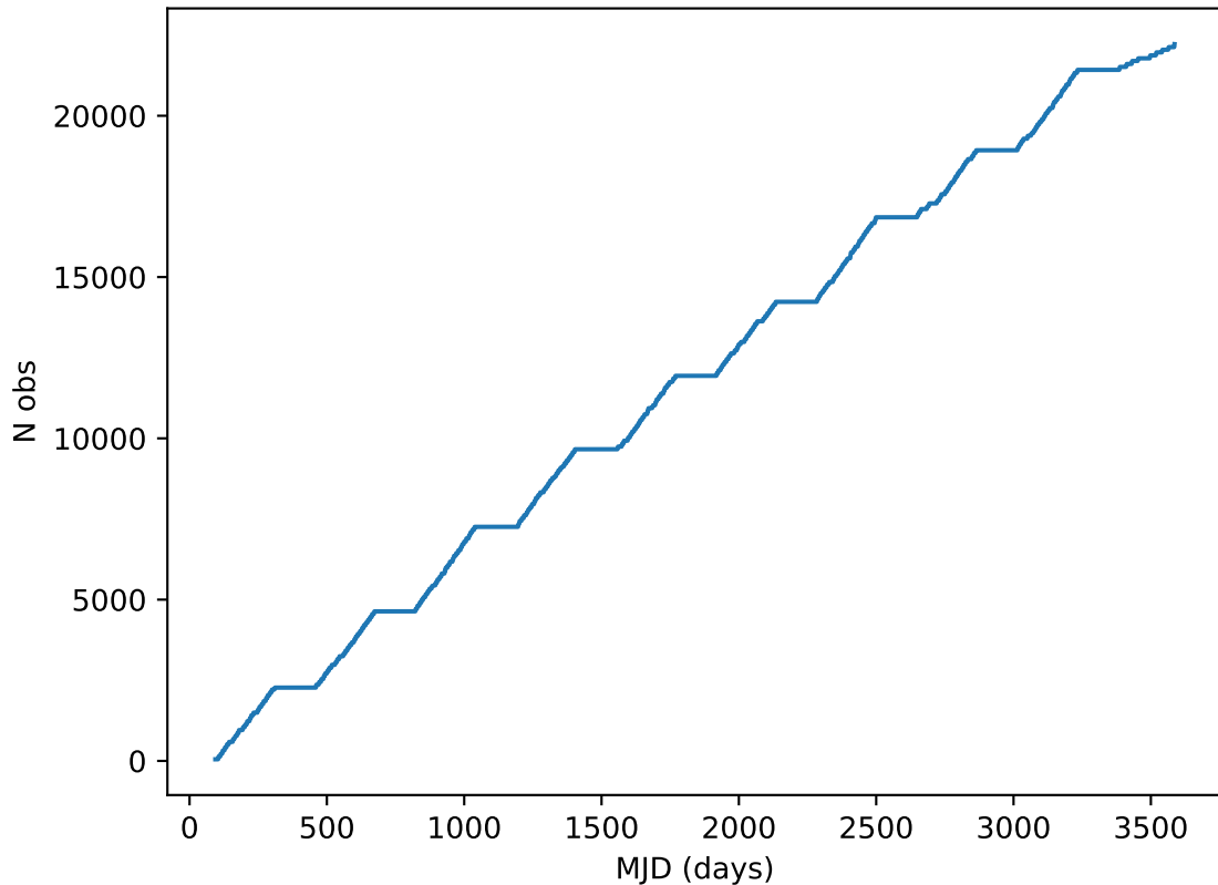
too_elab_r64_d3_ugrizy_v3.4_10yrs all bands: DD:ECDFS Cumulative NVisits
