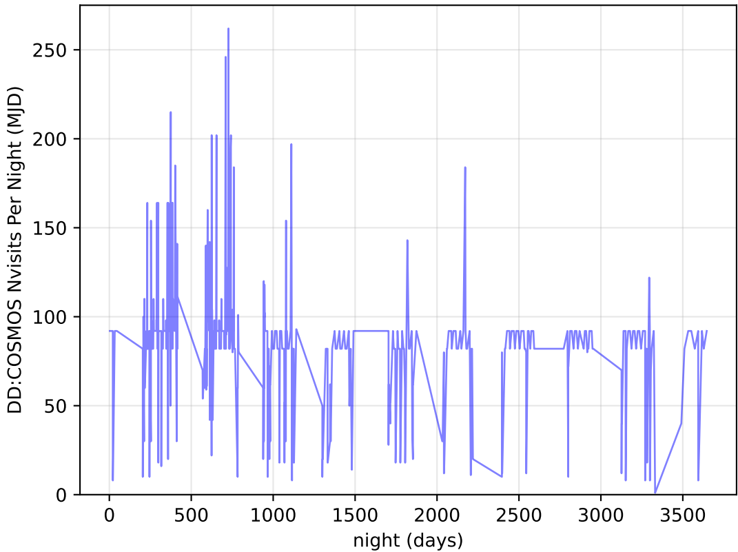
too_elab_r64_d3_ugrizy_v3.4_10yrs all bands: DD: COSMOS Nvisits Per Night
