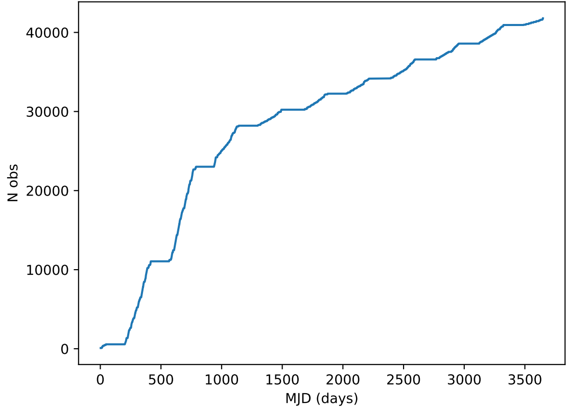
too_elab_r64_d3_ugrizy_v3.4_10yrs all bands: DD: COSMOS Cumulative NVisits
