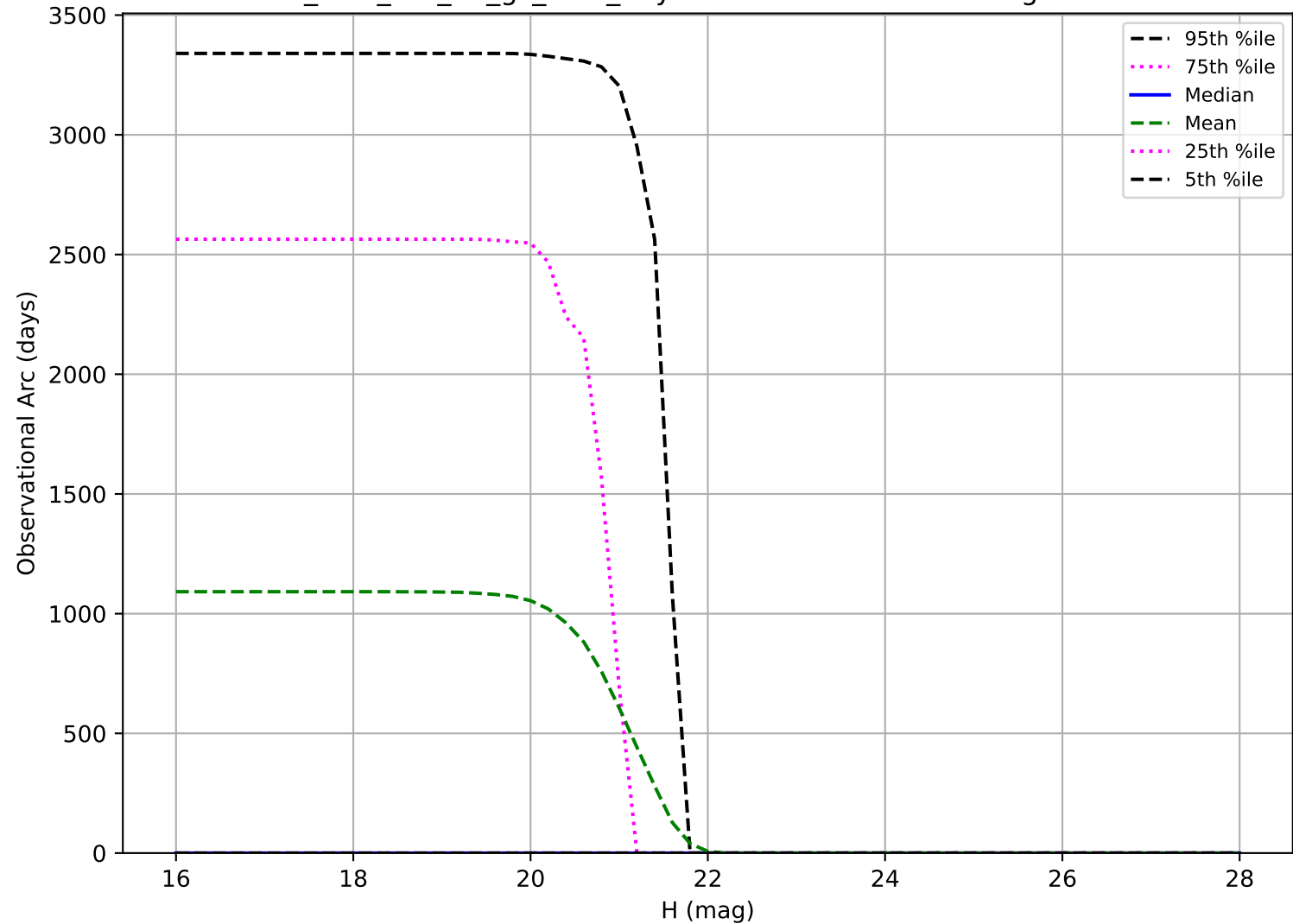
too_elab_r64_d3_gz_v3.4_10yrs: Observational Arc Length Vatira
