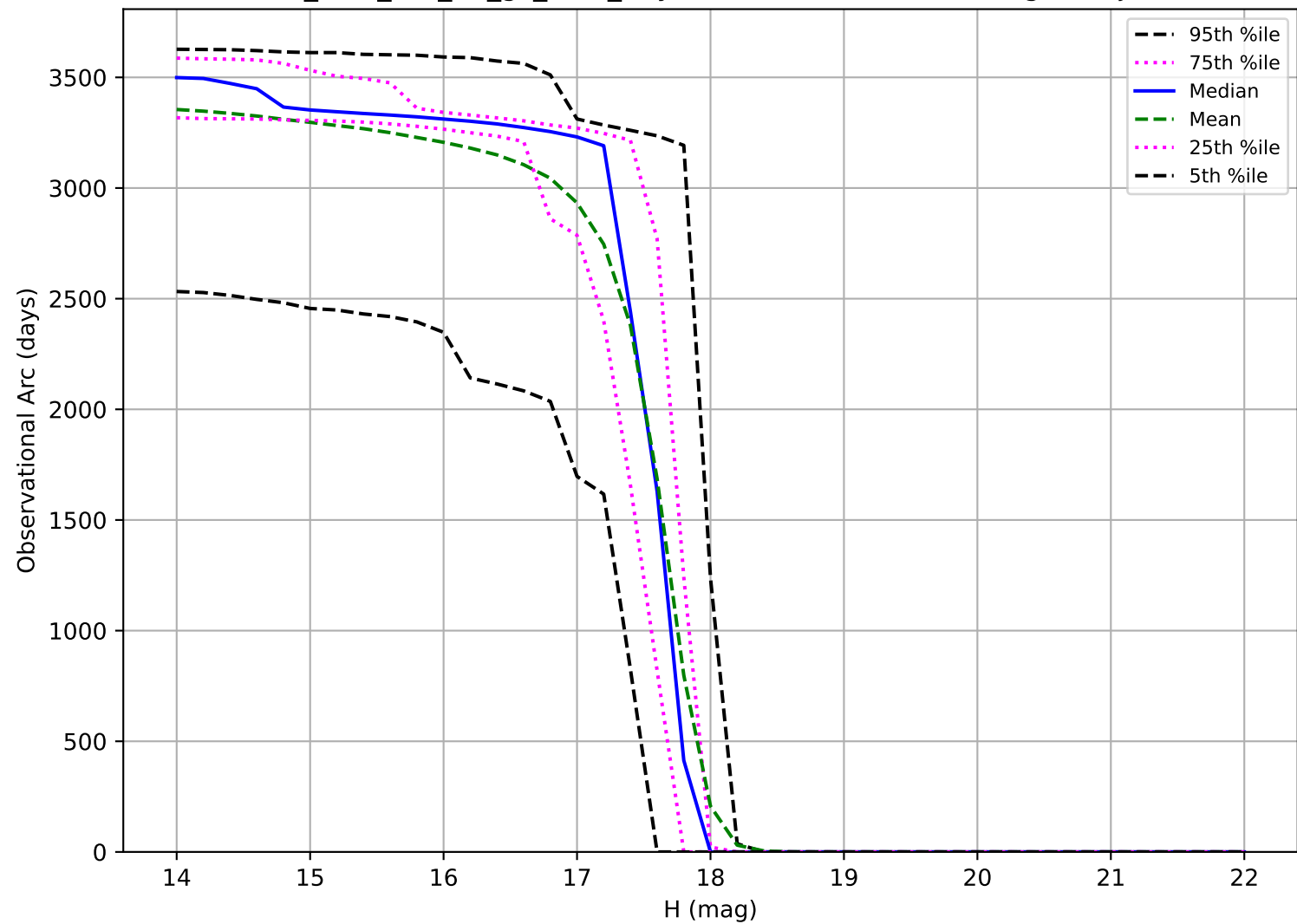
too_elab_r64_d3_gz_v3.4_10yrs: Observational Arc Length Trojan
